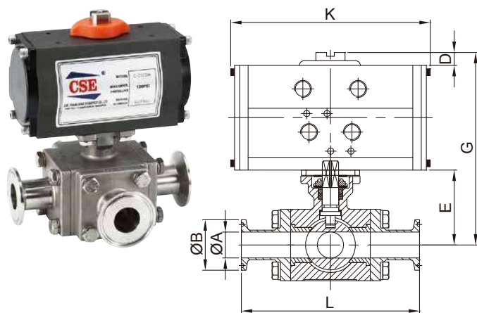
HIGH MOUNT PLATE DESIGN
