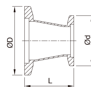
Conical Reducer
