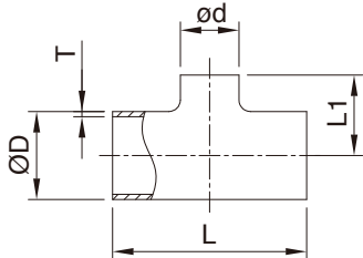
Reducing Tee
