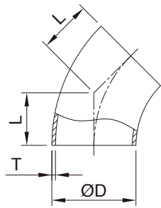
45° Short Elbow
